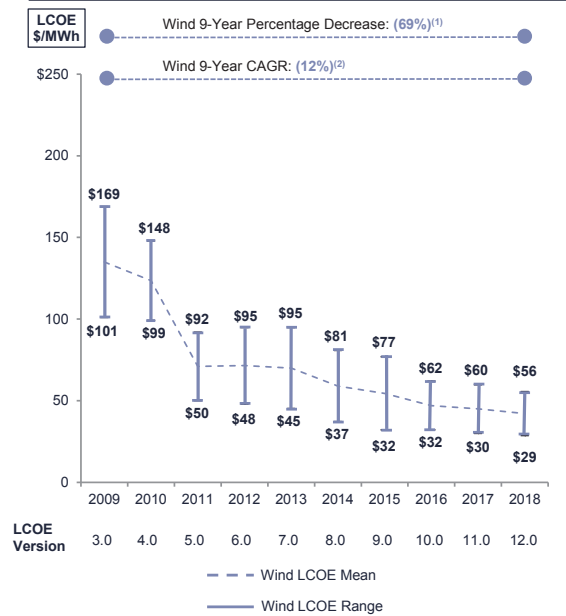
Unsubsidized Wind LCOE
